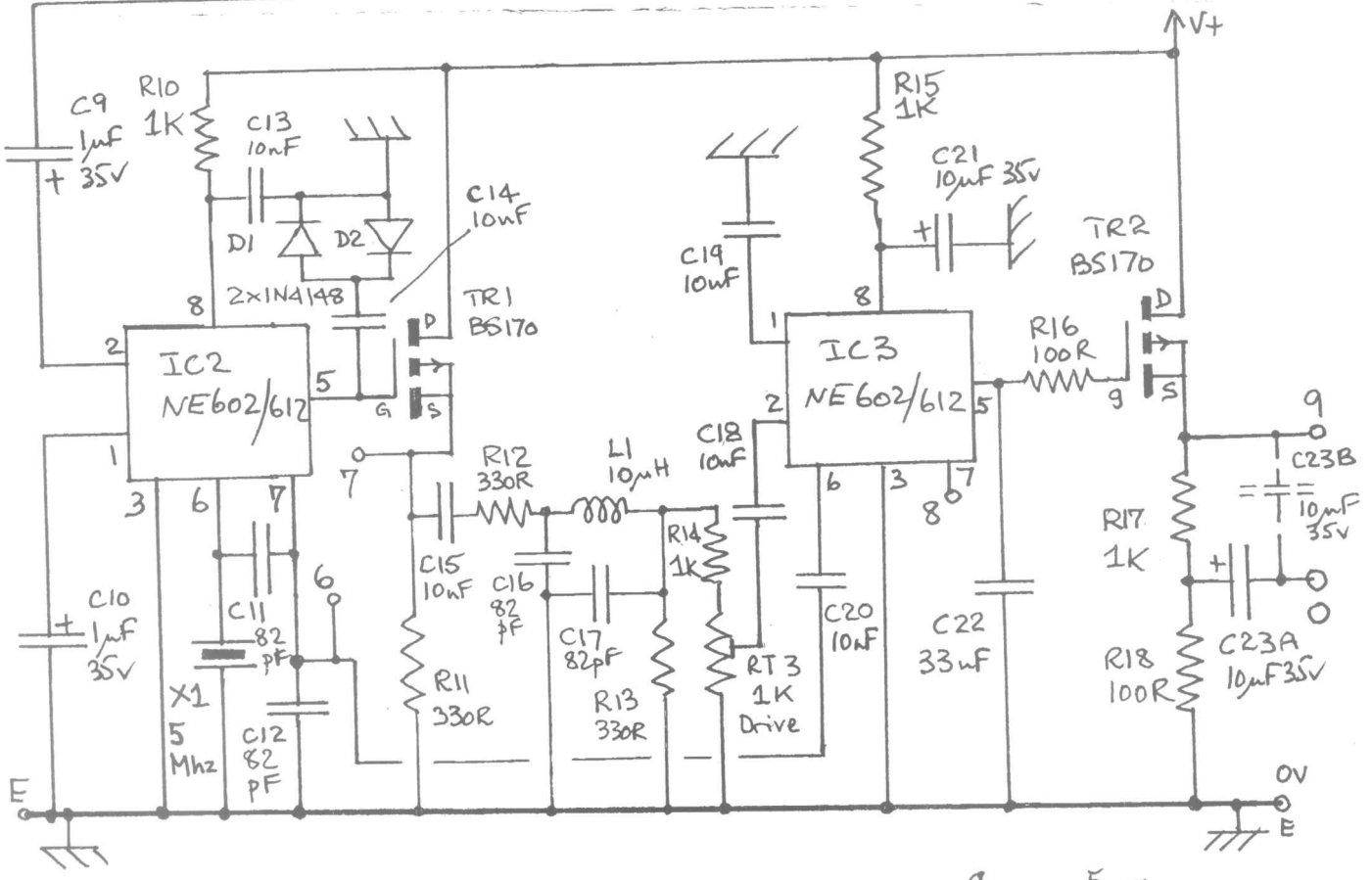
FIG 3 : SPEECH PROCESSOR CIRCUIT
